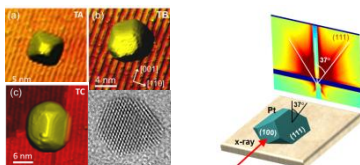
Fig. 1. (a-c) STM images of micellar Pt NPs on TiO 2 (110) acquired at RT after annealing in UHV at 1000°C. (d) High resolution TEM image of a Pt NP deposited on SiO 2 /Si obtained at RT after annealing at 800°C in H 2 . (e) GISAXS data from shape-selected Pt NPs on SrTiO 3 (110) acquired in H 2 at 700°C.
